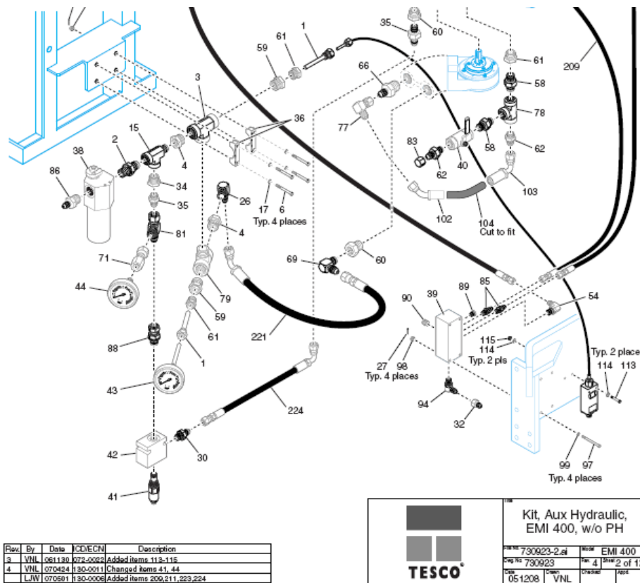
Figure 1 – EMI 400 Lube system
