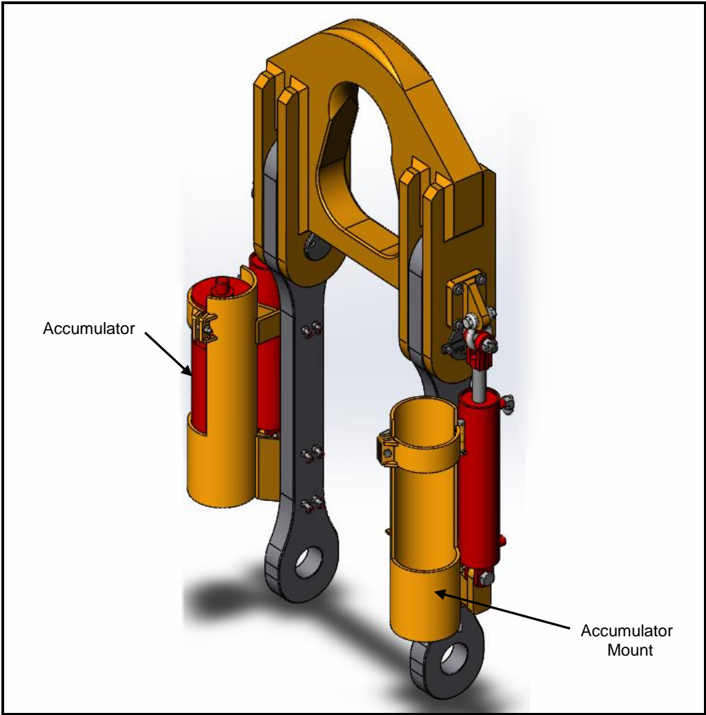
Figure 1: Olaer accumulator mount
