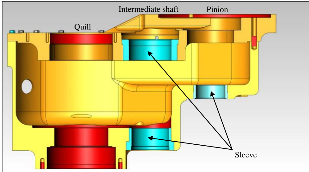
Figure 1: EMI-400 gearbox showing pre-sleeved bores
