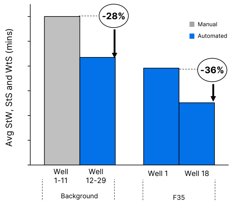
Manual vs. Automated Lateral Connection Times Using SmartDRILL®
